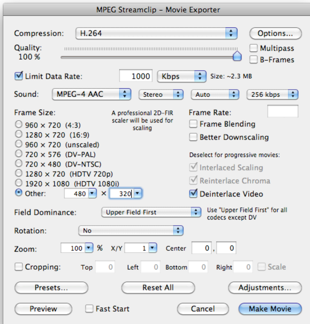
Figure 2: H.264 Compression
